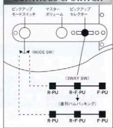
CONTROLS & SWITCH
