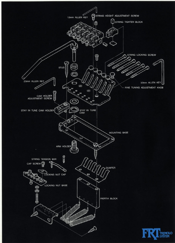
FRT-4 TREMOLO SYSTEM
