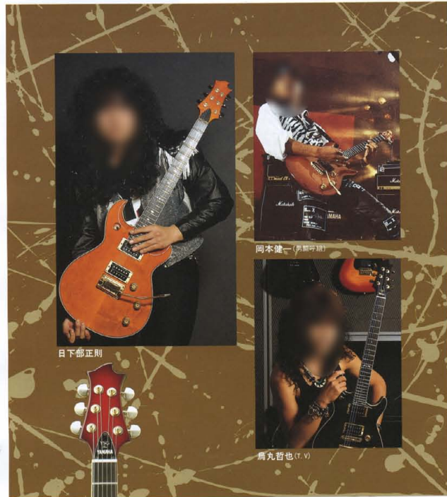
YSG-I ¥120,000 Body: Maple 2P (Top) + Mahogany 2P (Back), Bound Body Neck: Mahogany (Set in Body) Fingerboard: Bound Ebony 24F (350R Jim Dunlop #6100) Bridge: YSG-IG Pickups: "LIVE"-GHI (Alnico V) x2 Controls: Master Volume, Front P.U. Volume, Master Tone (Bi-Sound SW), 3P-Selector SW Scale: 628mm Hardware: Gold Finish: STB, VFS, SRS, SNS
